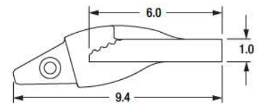
Side view of cast lips
