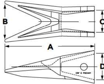
TYPE 5 - TWIN TIGER
