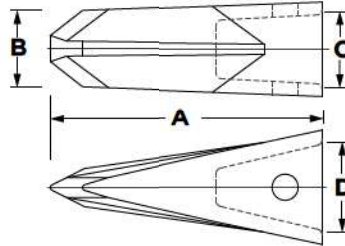
TYPE 11 - ROCK CHISEL
