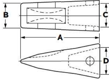
TYPE 3 - HEAVY LONG
