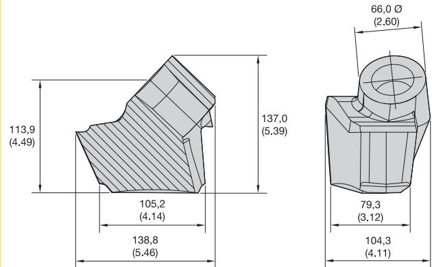
■ KPR302 Base • Right Hand
